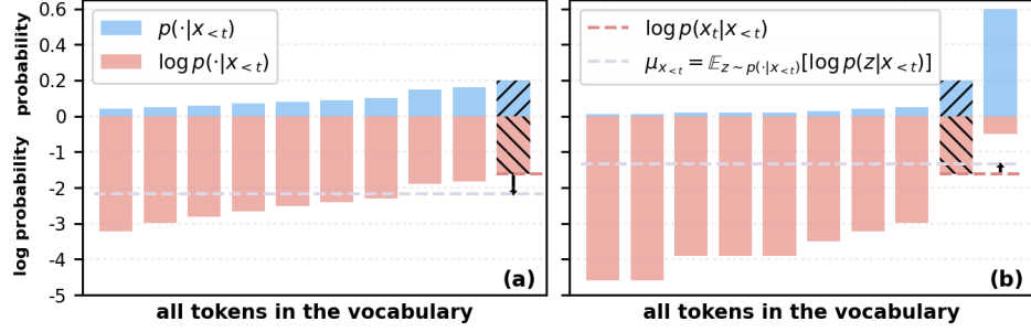
Figure 2: A conceptual example showcasing the idea of Min-K%++. (a) and (b) show two next token distributions for two different input token sequences ( x_{<t} , x_t ). The bars with the hatch pattern (‘//’) correspond to the target next token x_t . Existing methods often measure the exact next token probability of x_t (hatched bars), which fails to separate these two inputs due to the same probability (0.2). By comparison, Min-K%++ determines if x_t forms a mode or has relatively high probability by comparing \log p(x_t|x_{<t}) with \mu_{x_{<t}} ; the score is the difference between the red and pink dashed lines. See text for detailed discussion.
